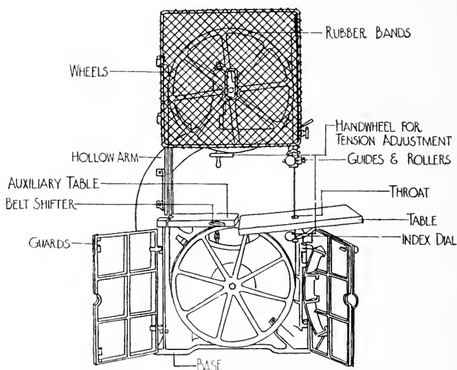
FIG. 182. BAND SAW WITH GUARDS.
